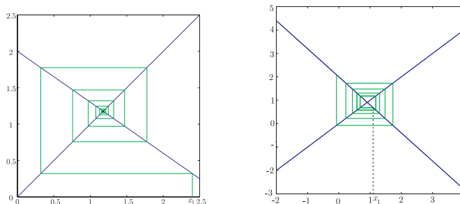
Figure 1: Stability and instability of the price
