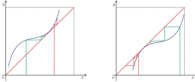
Figure 4: Semistable fixed points
