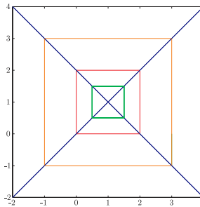
Figure 2: Stable but not asymptotically stable orbits
