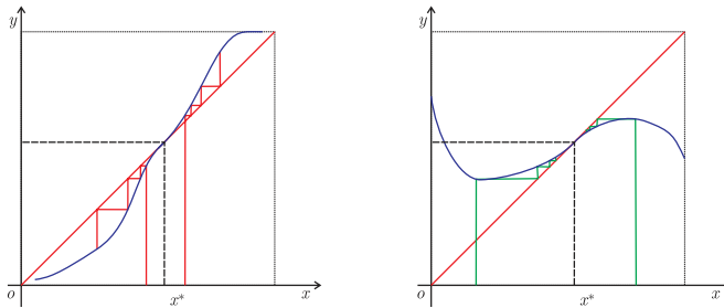
Figure 5: Unstable and stable fixed points in the case f'(x^*) = 1 and f''(x^*) = 0
