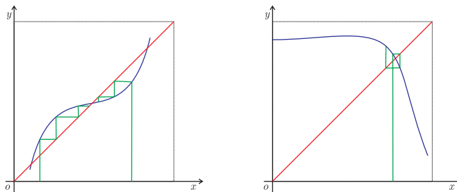
Figure 3: Asymptotically stable and unstable hyperbolic fixed points
