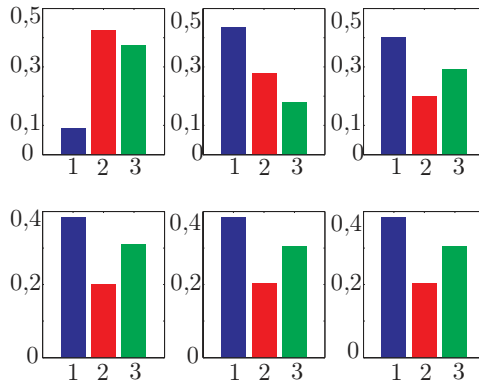
Figure 7: Convergence of iterates for a stochastic matrix
